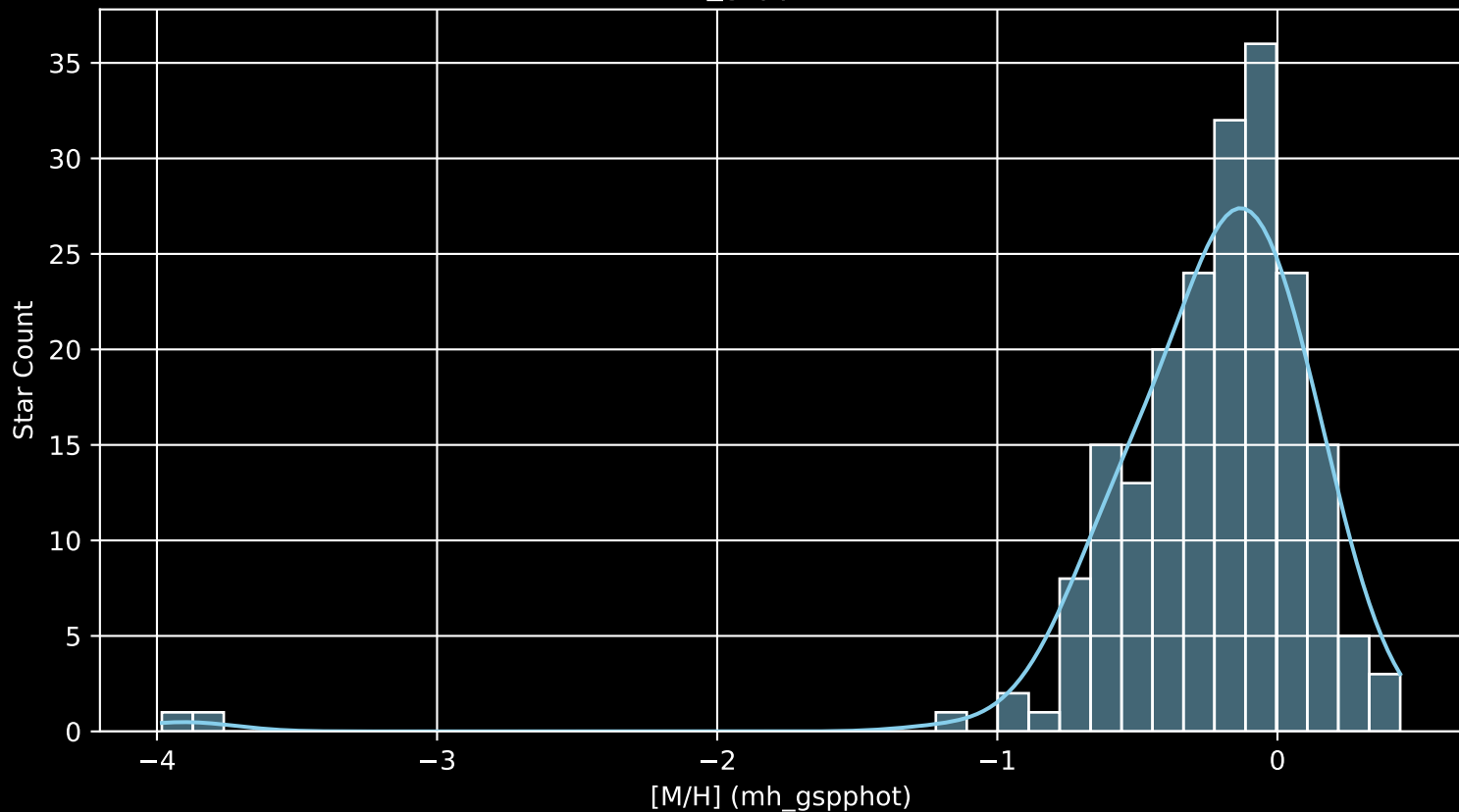
APOGEE DR17 Field: [186-55 [M/H] (mh_gspphot) (n= 201)
