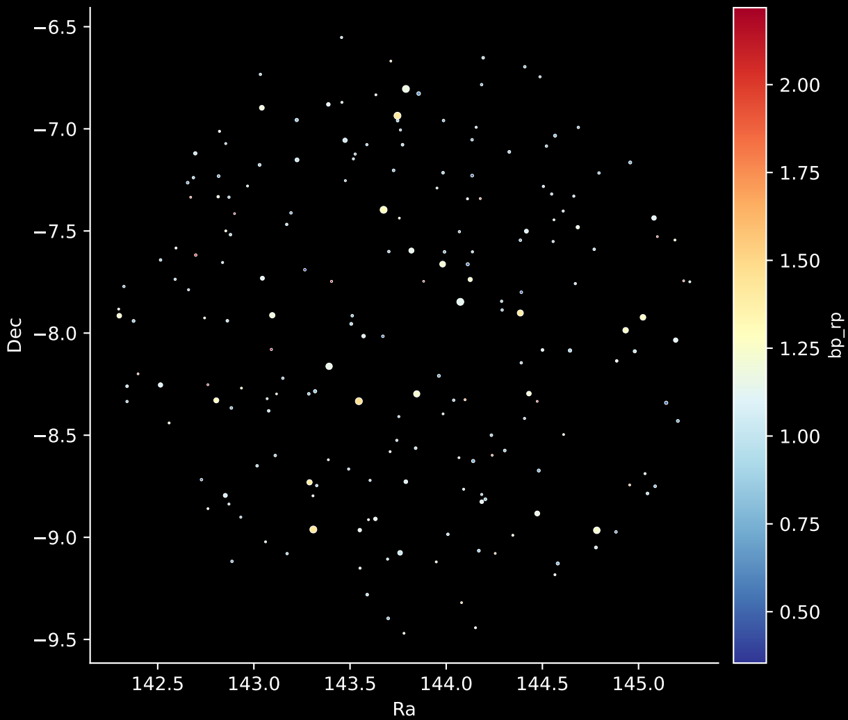
APOGEE DR17 Field: [186-55] Stars: 202
