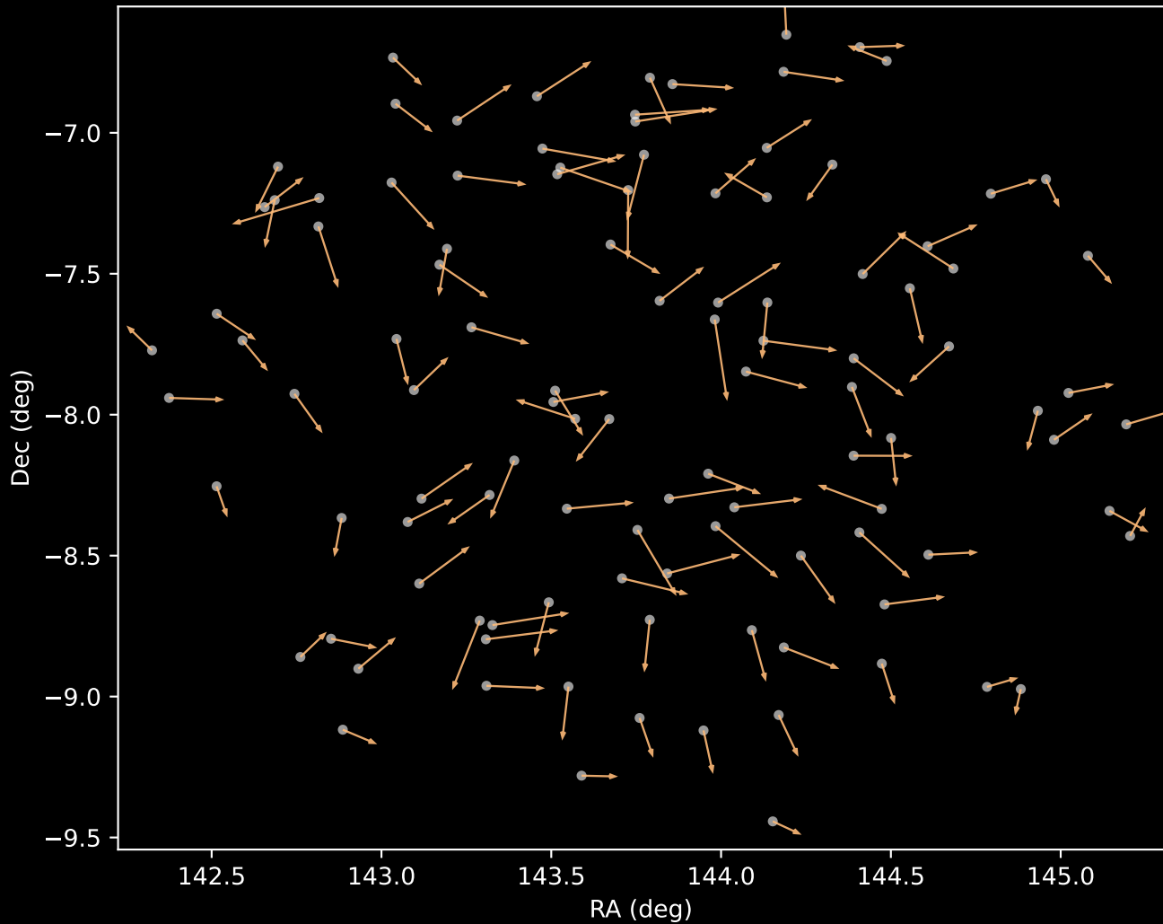
APOGEE DR17 Cluster 3 Proper Motion Vectors (n=108)
