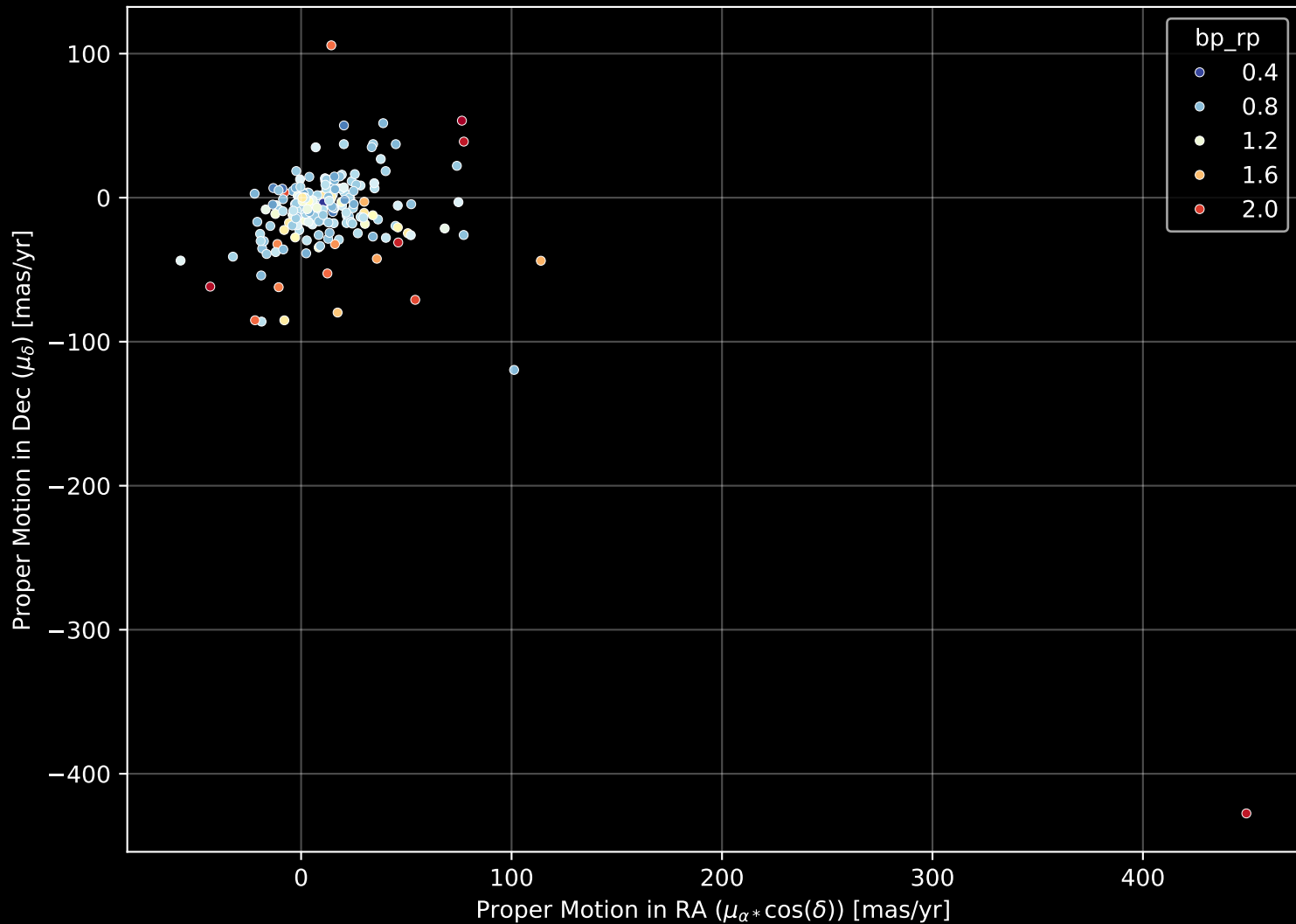
APOGEE DR17 Field: [186-55] Proper Motion Diagram (n= 202)
