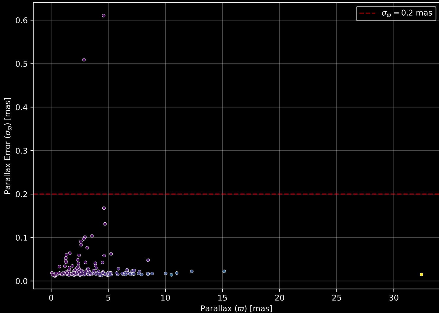
APOGEE DR17 Field: [186-55] Parallax Quality (n= 202)
