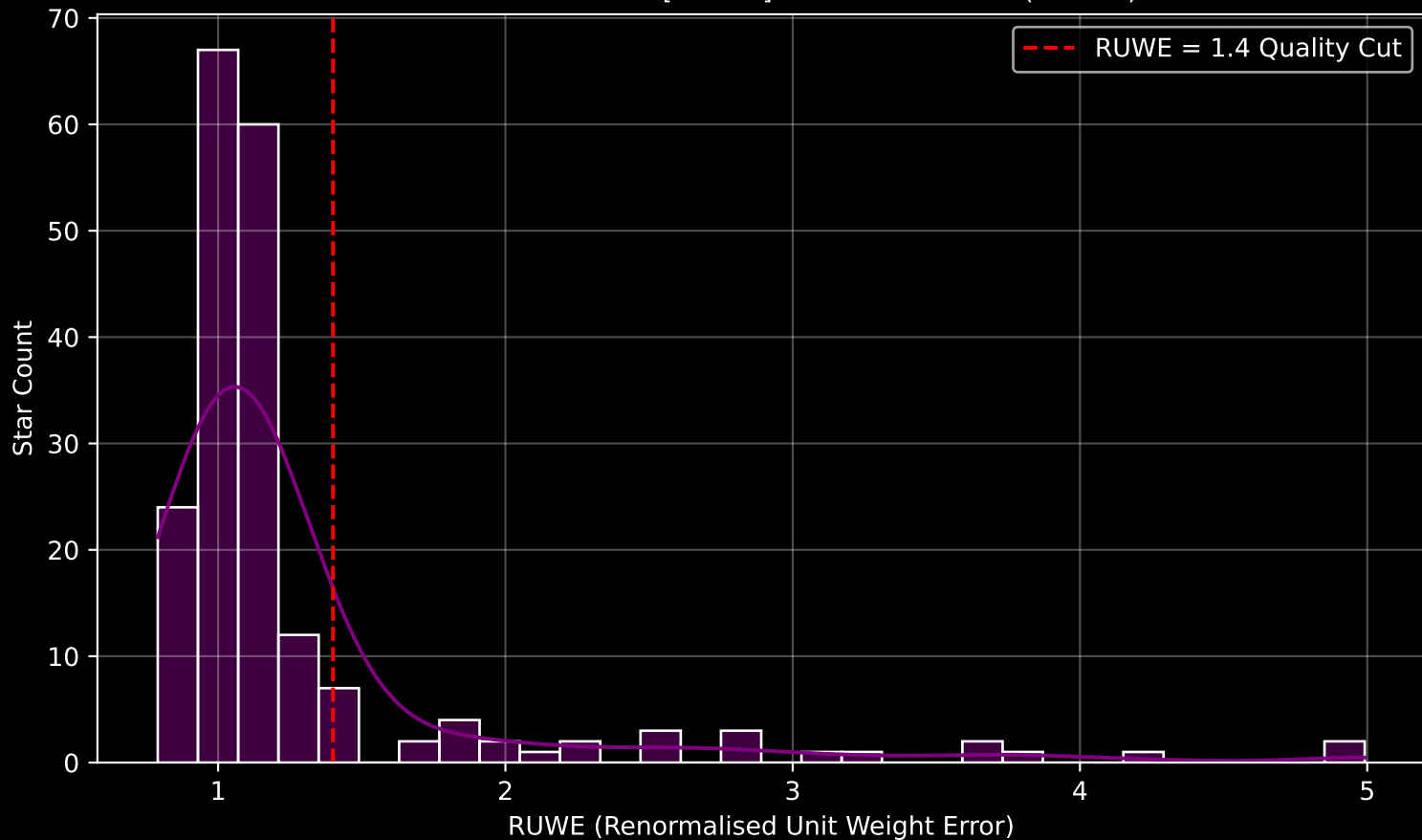
GAPOGEE DR17 Field [186-55] RUWE Distribution (n= 195)
