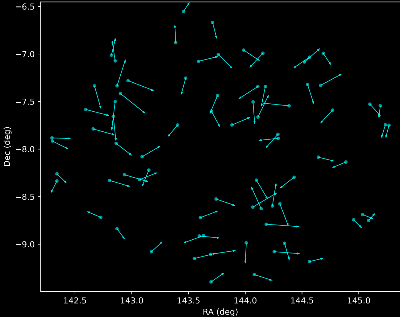
APOGEE DR17 Noise Stream Proper Motion Vectors (n=76)
