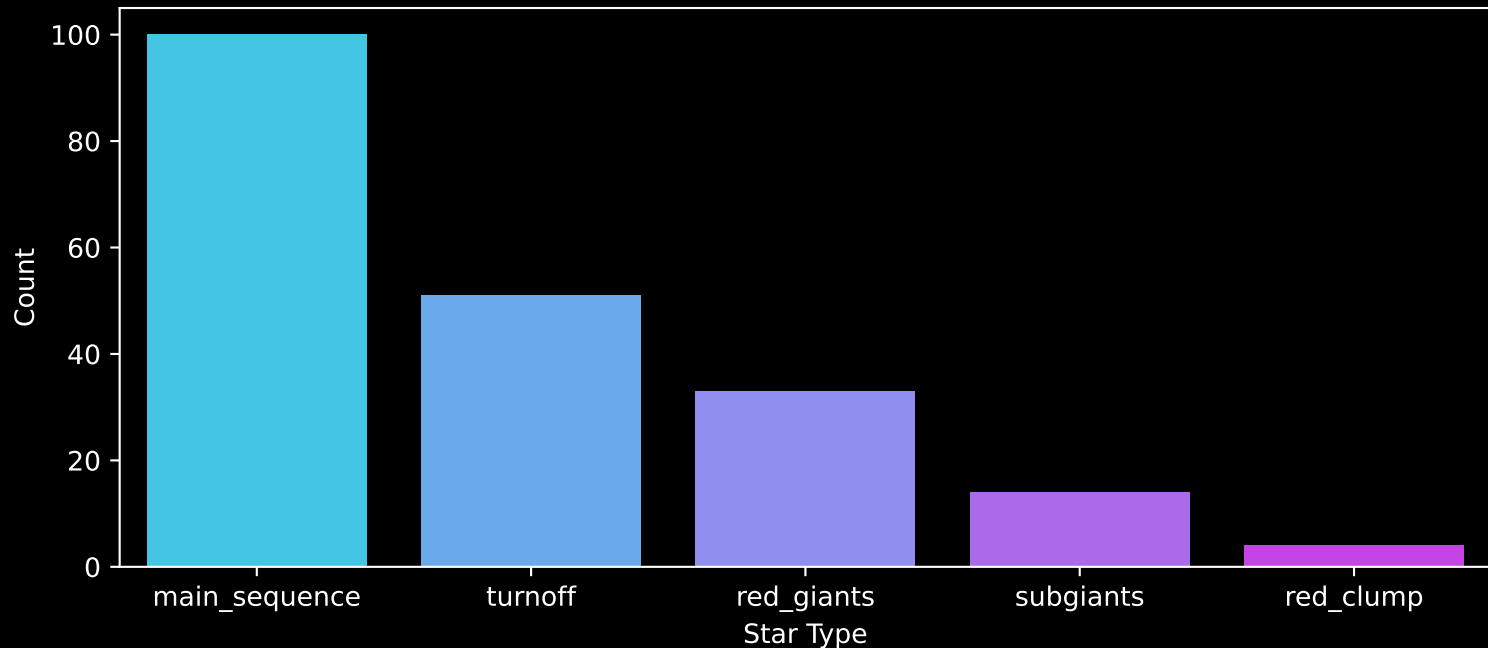
APOGEE DR17 Field: [186-55] Count plot of Star Type
